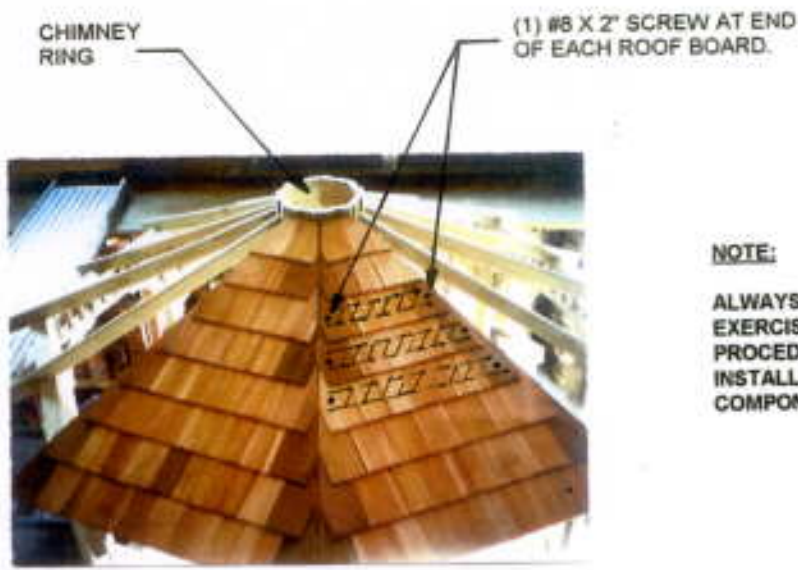
FIGURE 22: ROOF SECTION FASTENING
